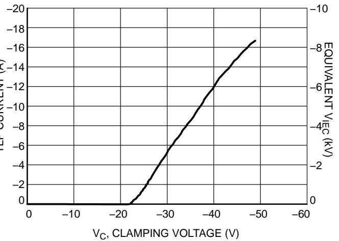
Figure 10. Typical Negative TLP IV Curve
