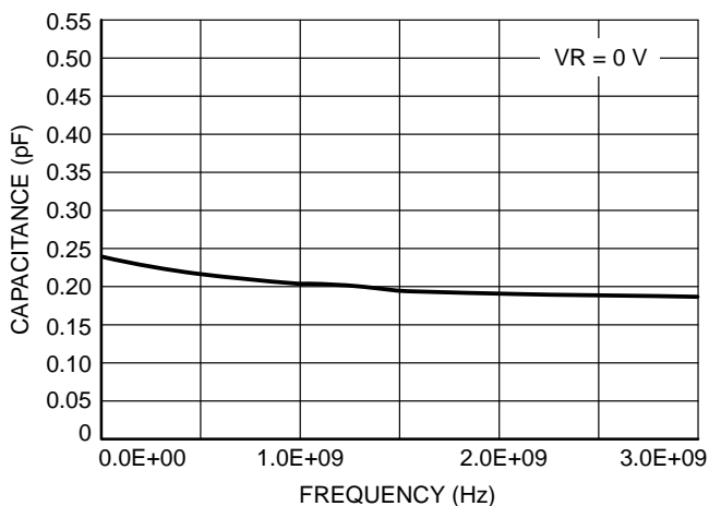
Figure 6. Typical Capacitance Over Frequency
