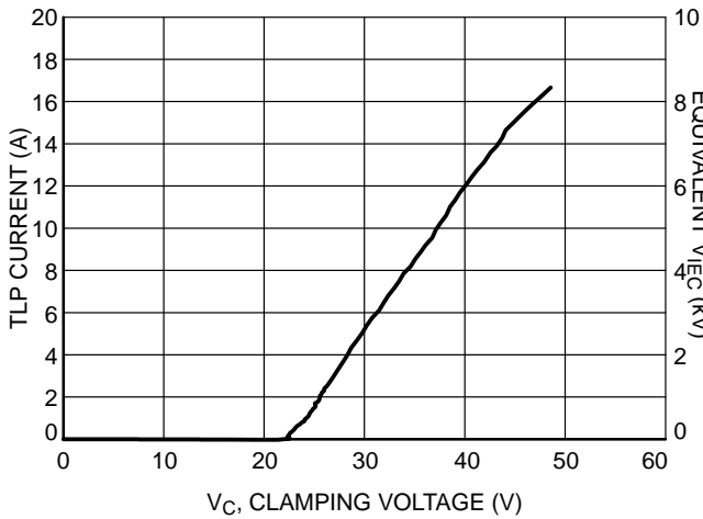
Figure 9. Typical Positive TLP IV Curve
