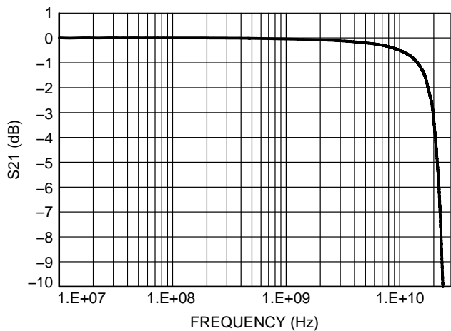
Figure 5. Typical Insertion Loss
