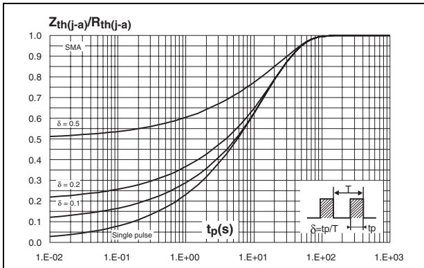
Figure 7. Relative variation of thermal impedance junction to ambient versus pulse duration - epoxy printed circuit board, eCu = 35 µm, recommended pad layout (SMA)
