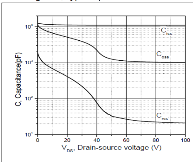
Figure 3, Typ. capacitances
