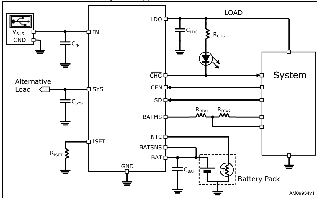
Figure 1. Application schematic
