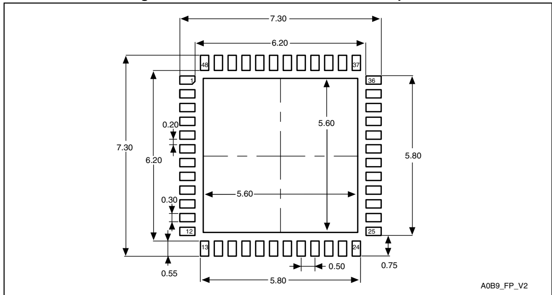
Figure 54. UFQFPN48 Recommended footprint
