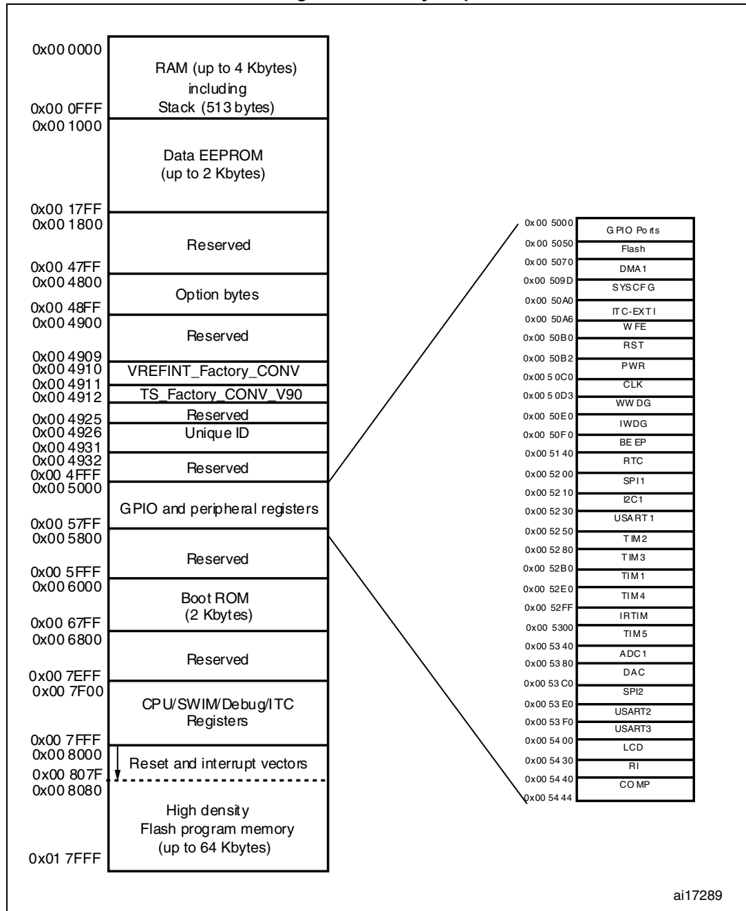
Figure 9. Memory map
