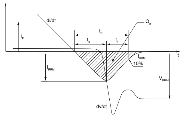
Figure 29. Diode reverse recovery waveform
