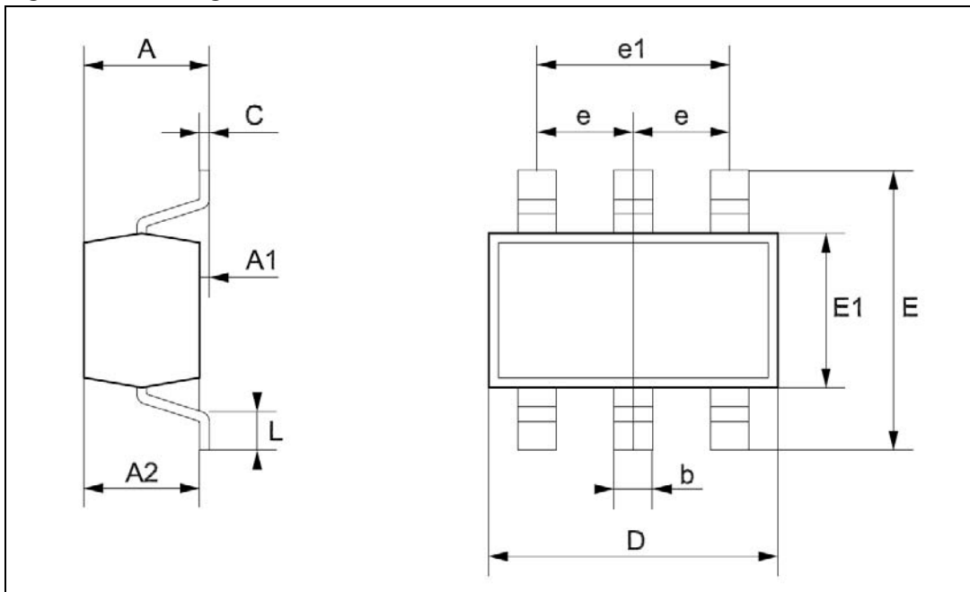
Figure 13. Package dimensions
