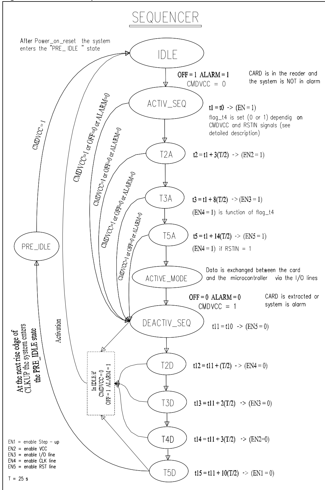
Figure 10. ST8004 Sequencer
