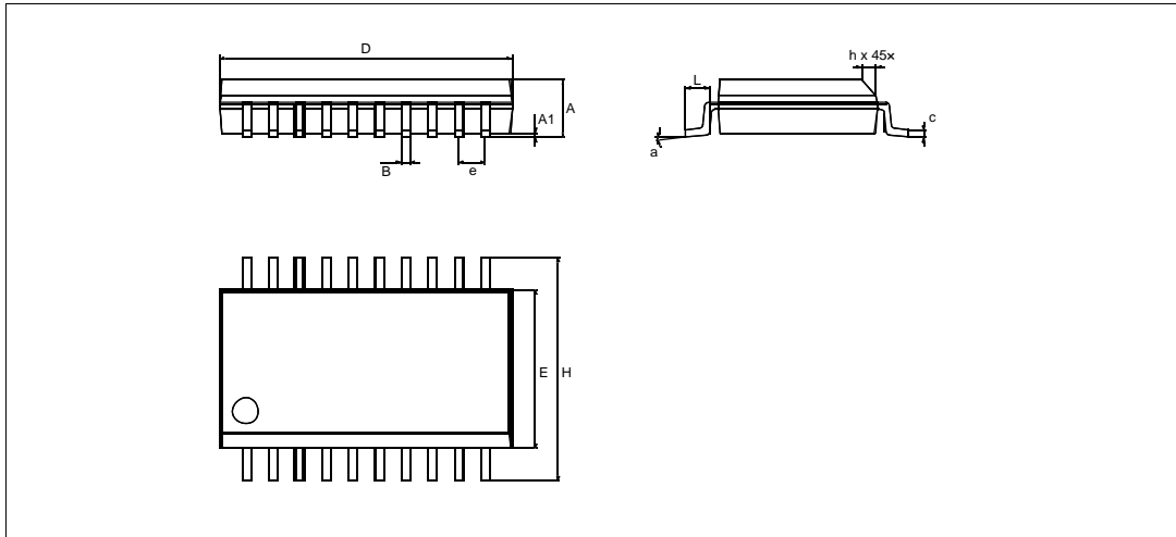
Figure 94. 20-pin plastic small outline package, 300-mil width, package outline
