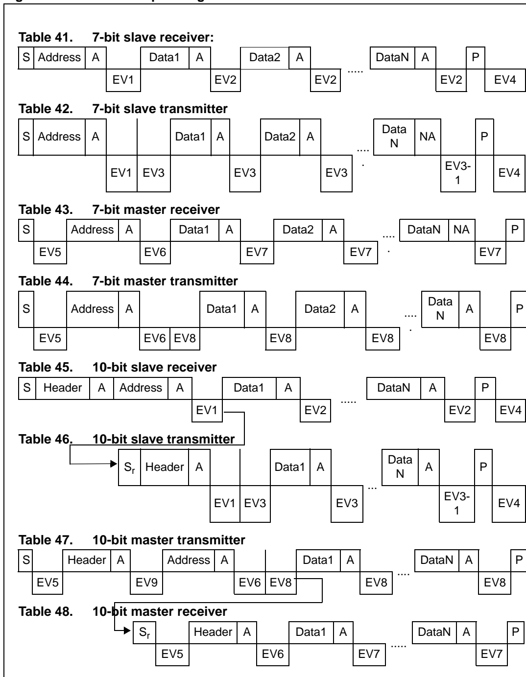
Figure 57. Transfer sequencing
