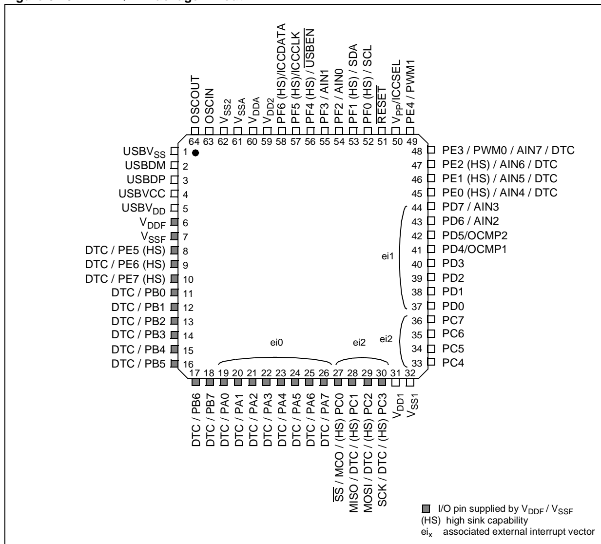
Figure 6. 64-Pin TQFP Package Pinout
