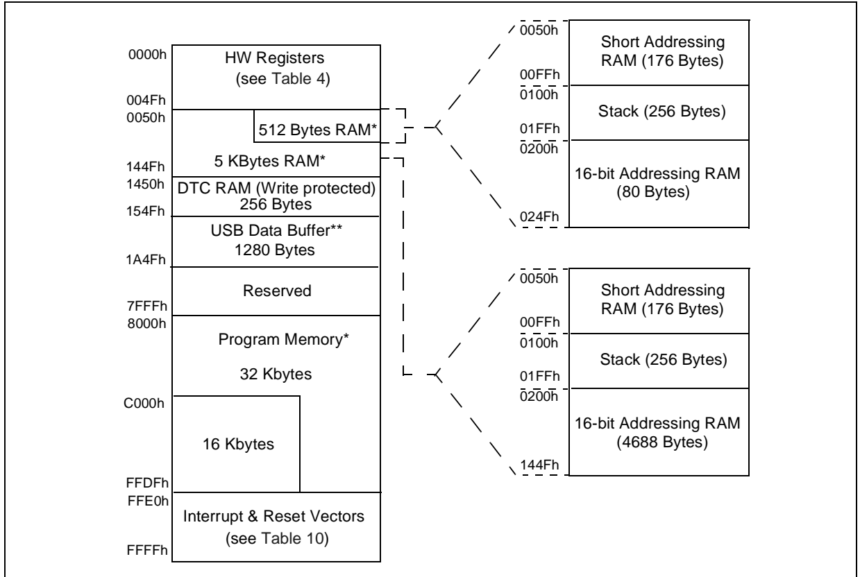
Figure 11. Memory Map
