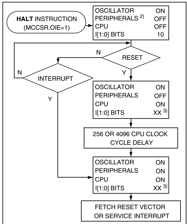
Figure 28. ACTIVE-HALT Mode Flow-chart
