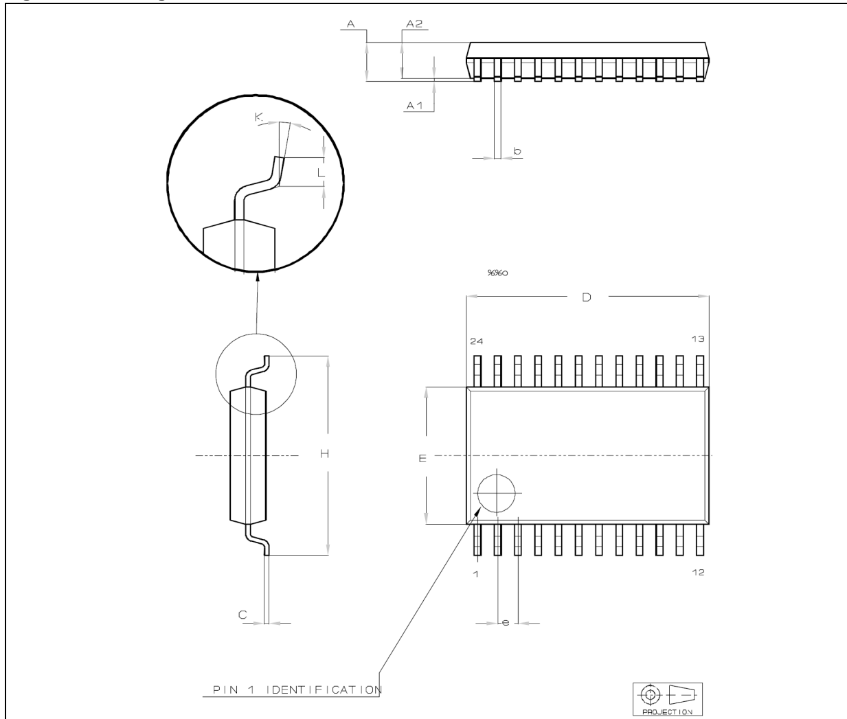
Figure 7. Package Dimensions
