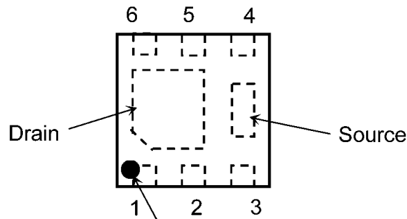
Polarity marking (on the top)
