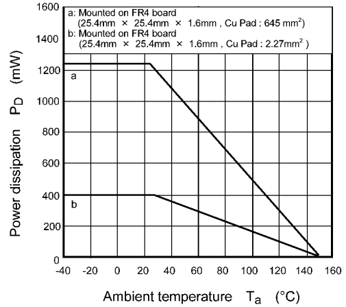
Fig. 8.14 P_D - T_a
