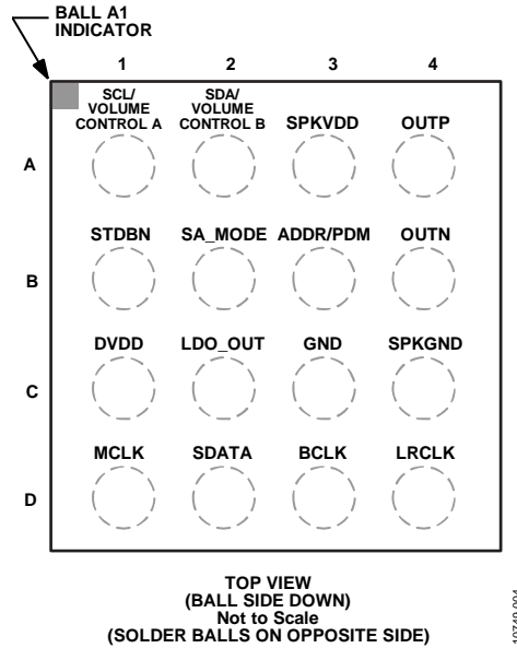
Figure 4. Pin Configuration
