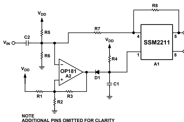
Figure 47. Automatic Shutdown Circuit
