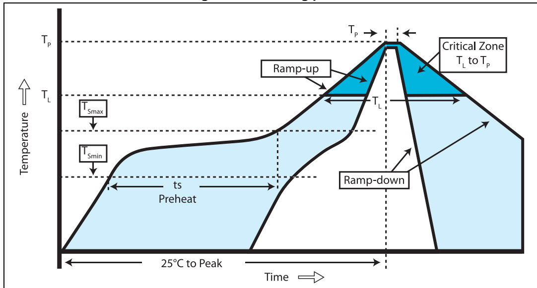
Figure 6. Soldering profile
