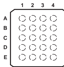
GQN OR ZQN PACKAGE (TOP VIEW)
