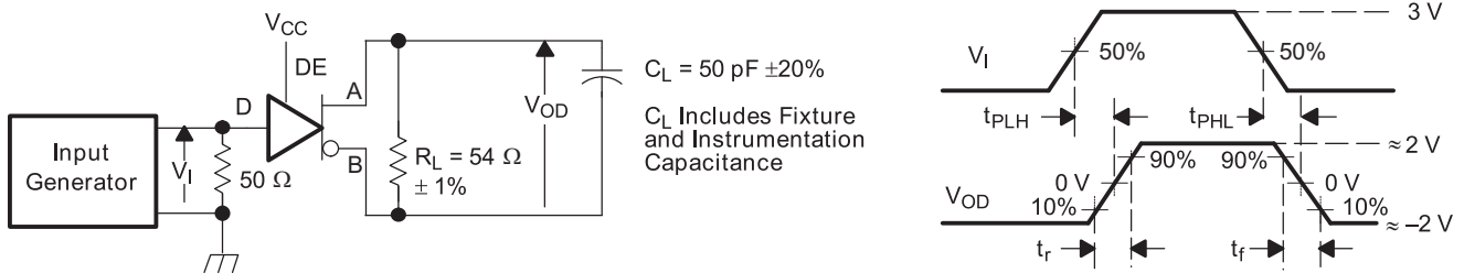
Figure 8. Measurement of Driver Differential Output Rise and Fall Times and Propagation Delays
