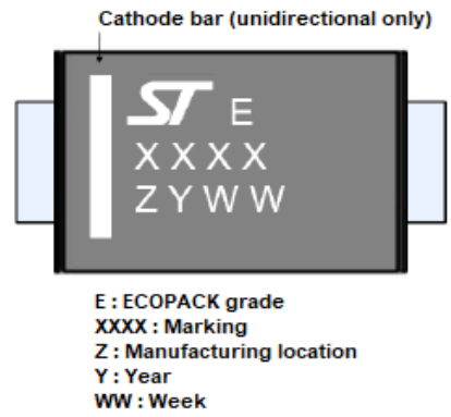
Figure 15. Marking layout
