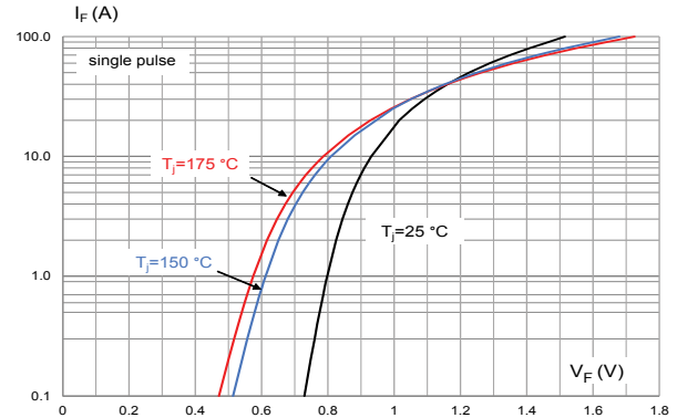
Figure 10. Peak forward voltage drop versus peak forward current
