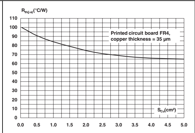
Figure 13. Thermal resistance junction to ambient versus lead copper surface under each lead
