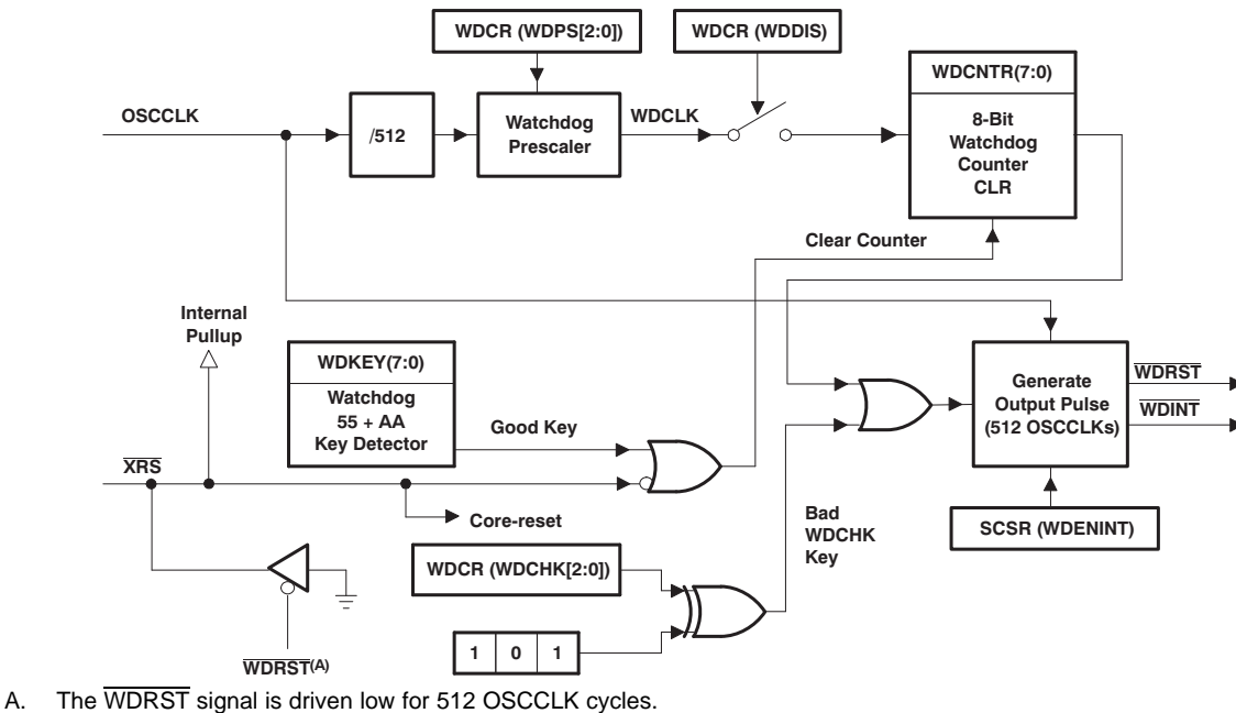
Figure 3-11. Watchdog Module
