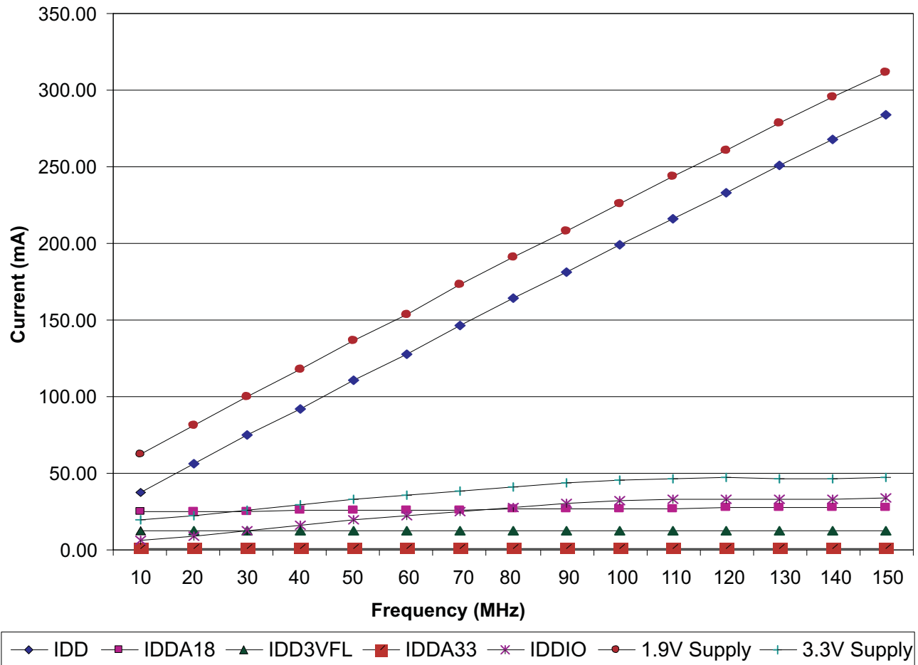
Figure 6-2. Typical Operational Current Versus Frequency for T_A = 25^\circ\text{C}
