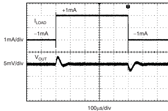
100\mu\text{s}/\text{div} ( C_L = 10 \mu\text{F} , I_{\text{OUT}} = 1 \text{ mA} )
