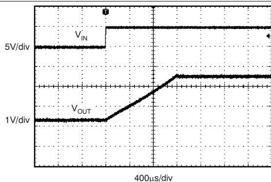
400\mu\text{s}/\text{div} (REF5025, C_L = 10\mu\text{F} )
