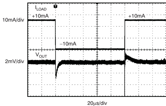
20\mu\text{s}/\text{div} ( C_L = 1 \mu\text{F} , I_{\text{OUT}} = 10 \text{ mA} )
