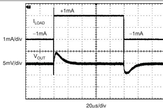
20\mu\text{s}/\text{div} ( C_L = 1 \mu\text{F} , I_{\text{OUT}} = 1 \text{ mA} )
