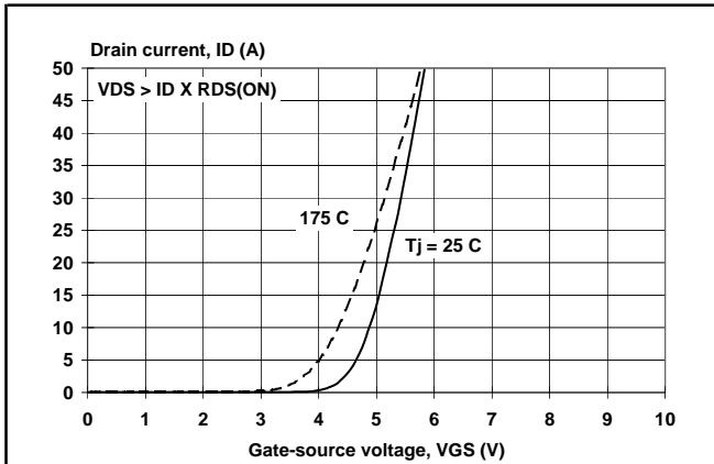
Fig. 7. Typical transfer characteristics. I_D = f(V_{GS}) ; parameter T_j
