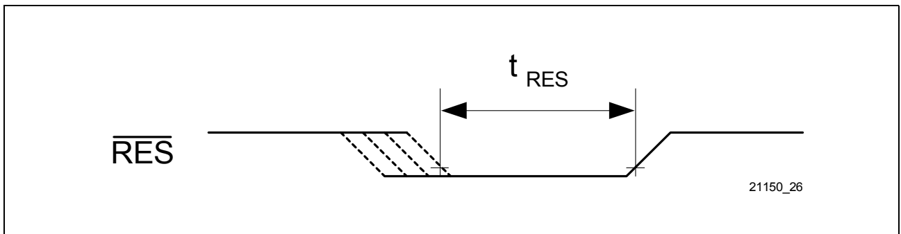
Figure 96 Reset Signal \overline{RES}
