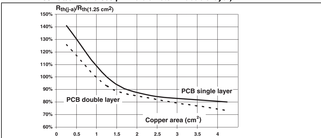
Figure 9. Thermal resistance variation versus copper area (35 \mu\text{m} layer thickness; 50vias/ \text{cm}^2 and 300 \mu\text{m} via diameter in double layer)
