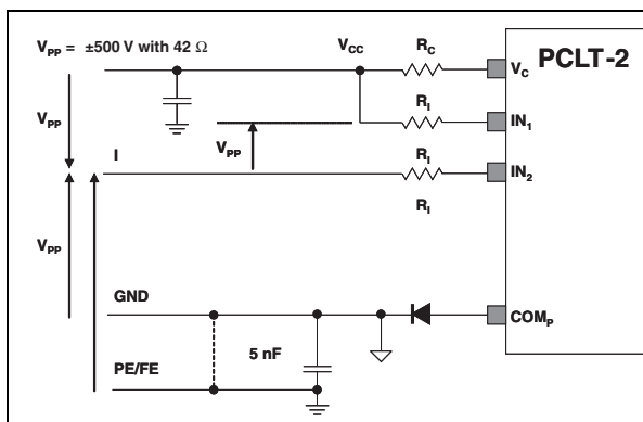
Figure 10. Input pin IN voltage surge test circuit
