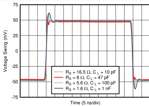
Figure 6-19. Small-Signal Transient Response
