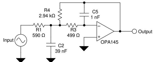
Figure 8-1. 25-kHz Low-Pass Filter
