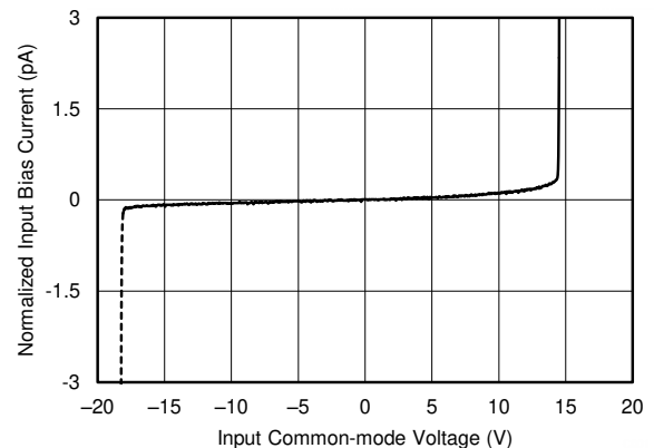
OPAx145 Precision JFET Technology Offers Excellent Linear Input Impedance
