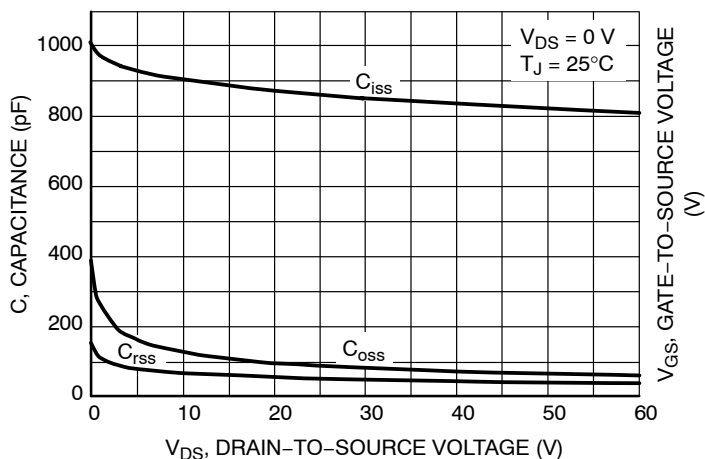
Figure 7. Capacitance Variation
