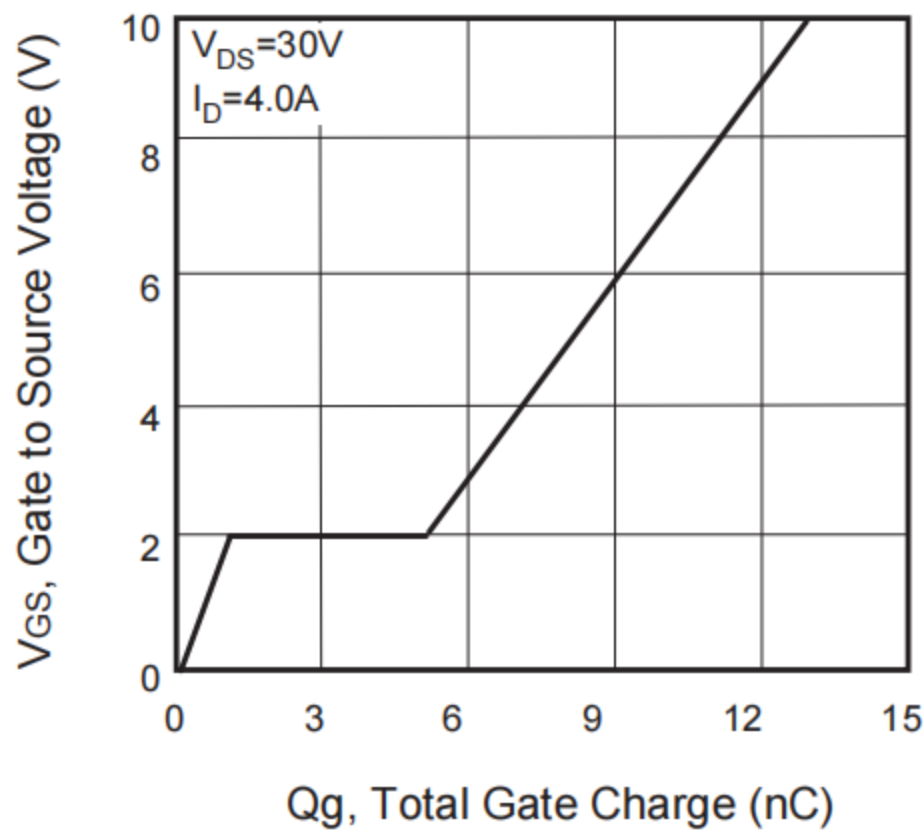
Figure 7. Gate Charge
