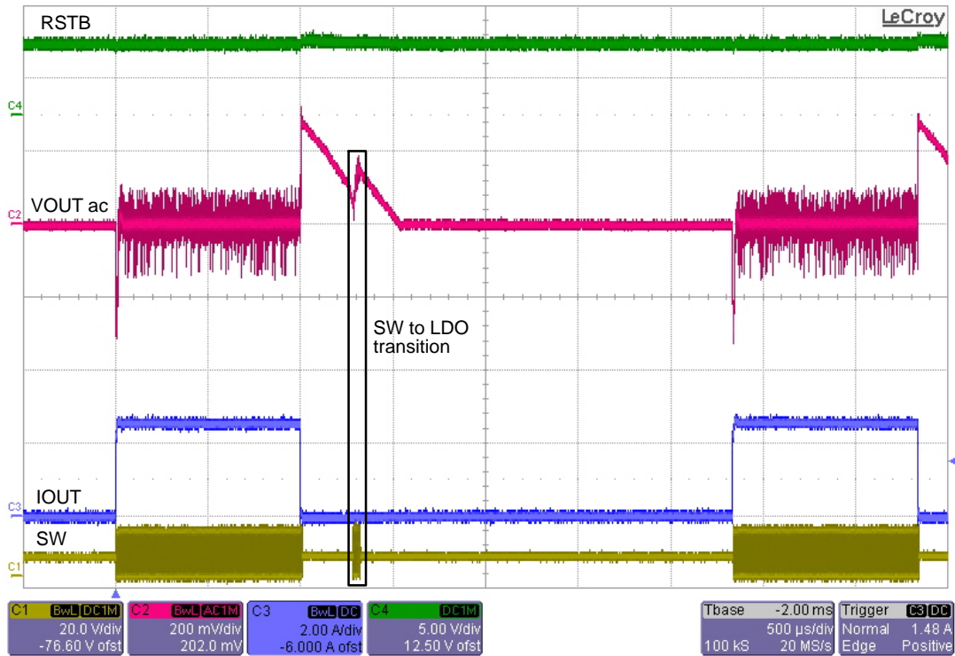
Figure 29. V_{IN} = 13\text{ V} , V_{OUT} = 5\text{ V} , 20 mA to 2.5 A at 1 A/μs – with Mode Transition
