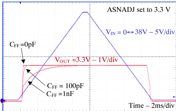
Figure 43. Startup Timing – Different C_{FF}
