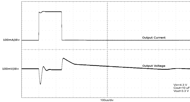
Figure 18. Load Transient Response (10 μF)
