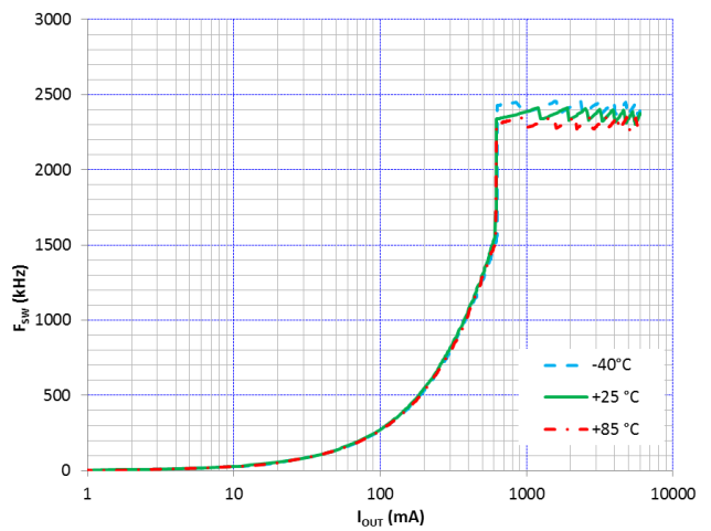
Figure 31. Switching Frequency vs I LOAD and Temperature, V OUT = 1.150 V
