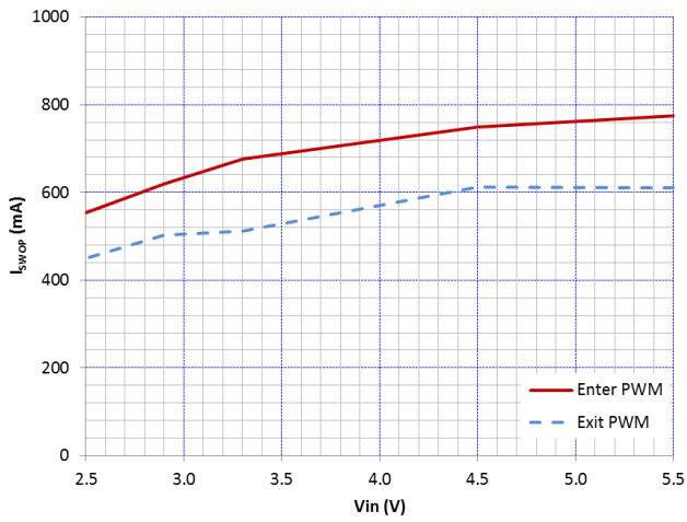
Figure 28. Switchover Point V OUT = 1.15 V
