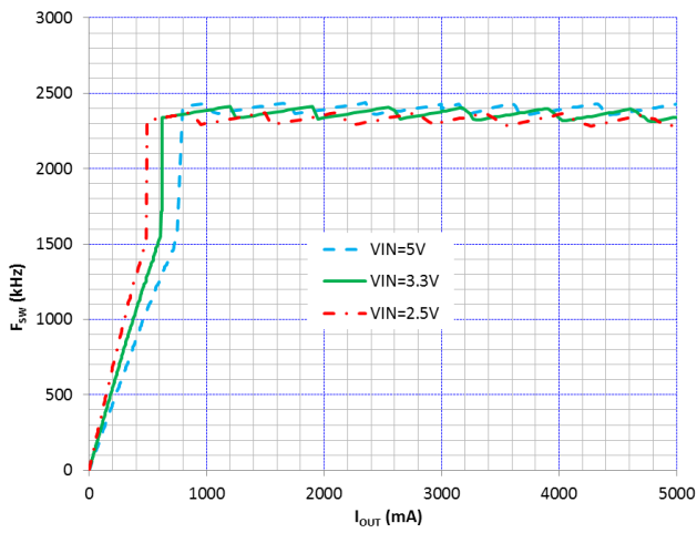
Figure 30. Switching Frequency vs I LOAD and V IN , V OUT = 1.150 V
