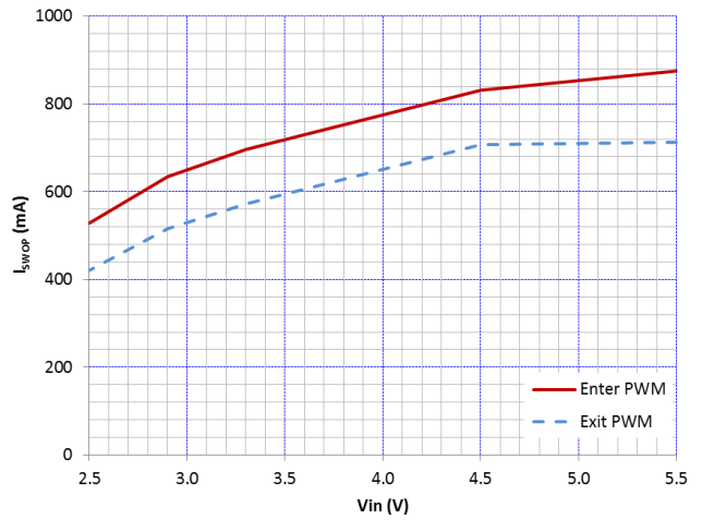
Figure 29. Switchover Point V OUT = 1.4 V
