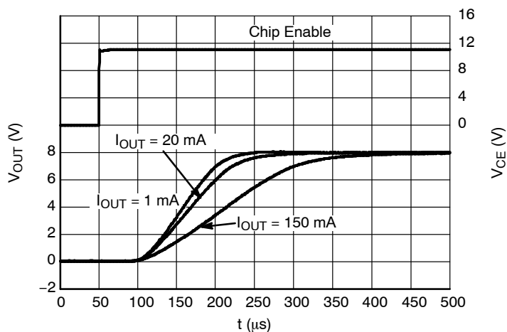
Figure 31. Start-up, 8.0 V Version, V_{IN} = 11.0 V
