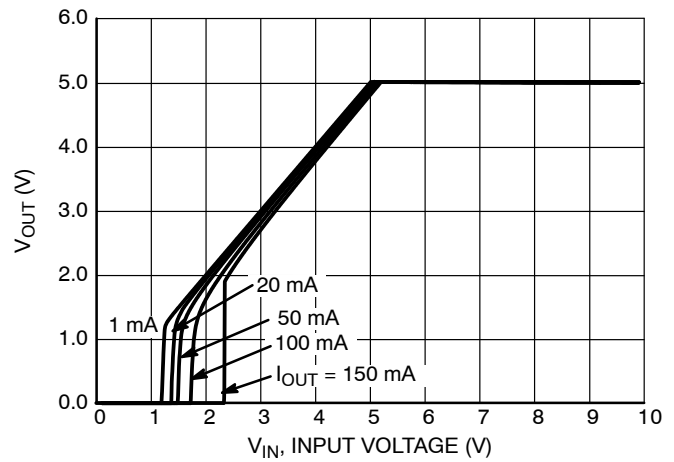
Figure 15. Output Voltage vs. Input Voltage, 5.0 V Version
