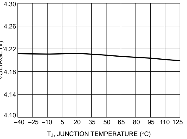
Figure 16. VB UVLO Rising Threshold vs. Junction Temperature
