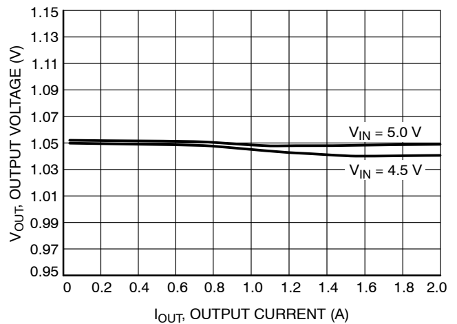
Figure 8. Load Regulation (1.05 V)
