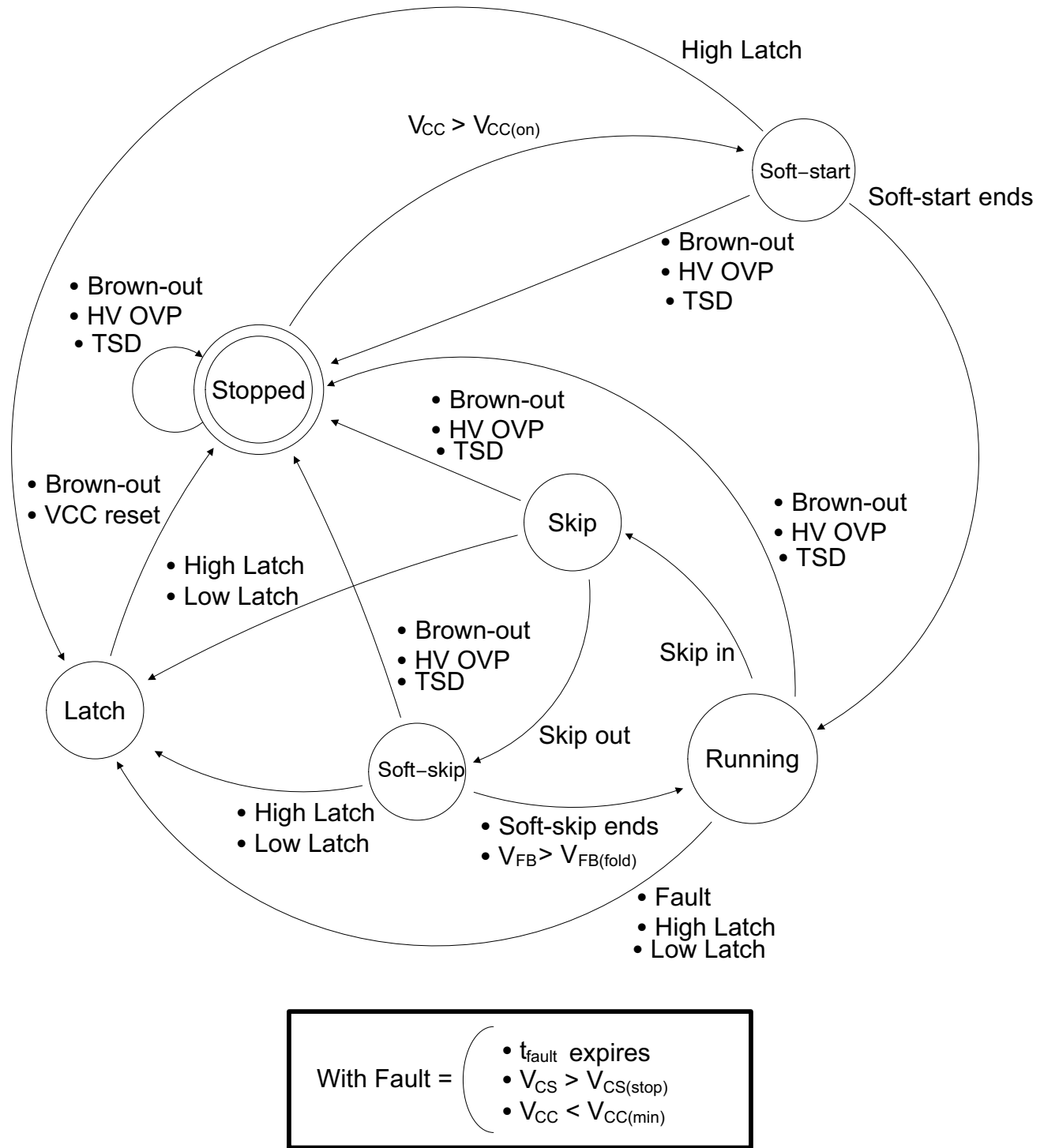
Figure 27. Controller Operation State Diagram (Latched Protection)
