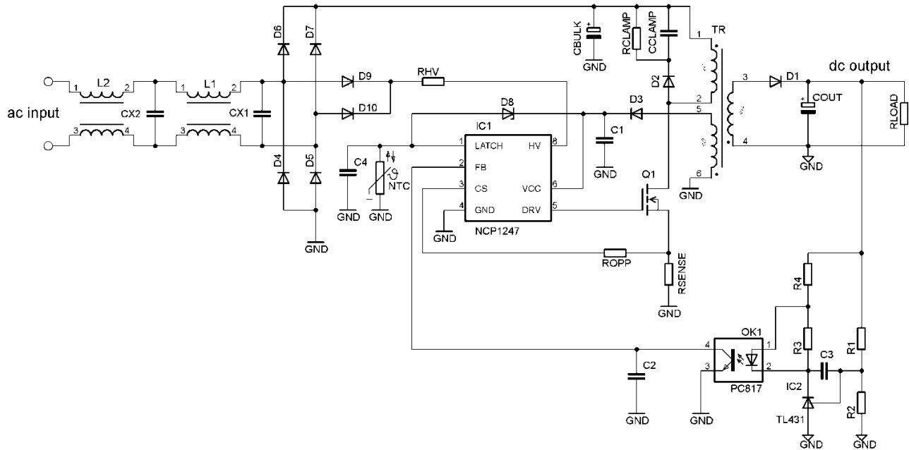
Figure 1. Flyback Converter Application Using the NCP1247
