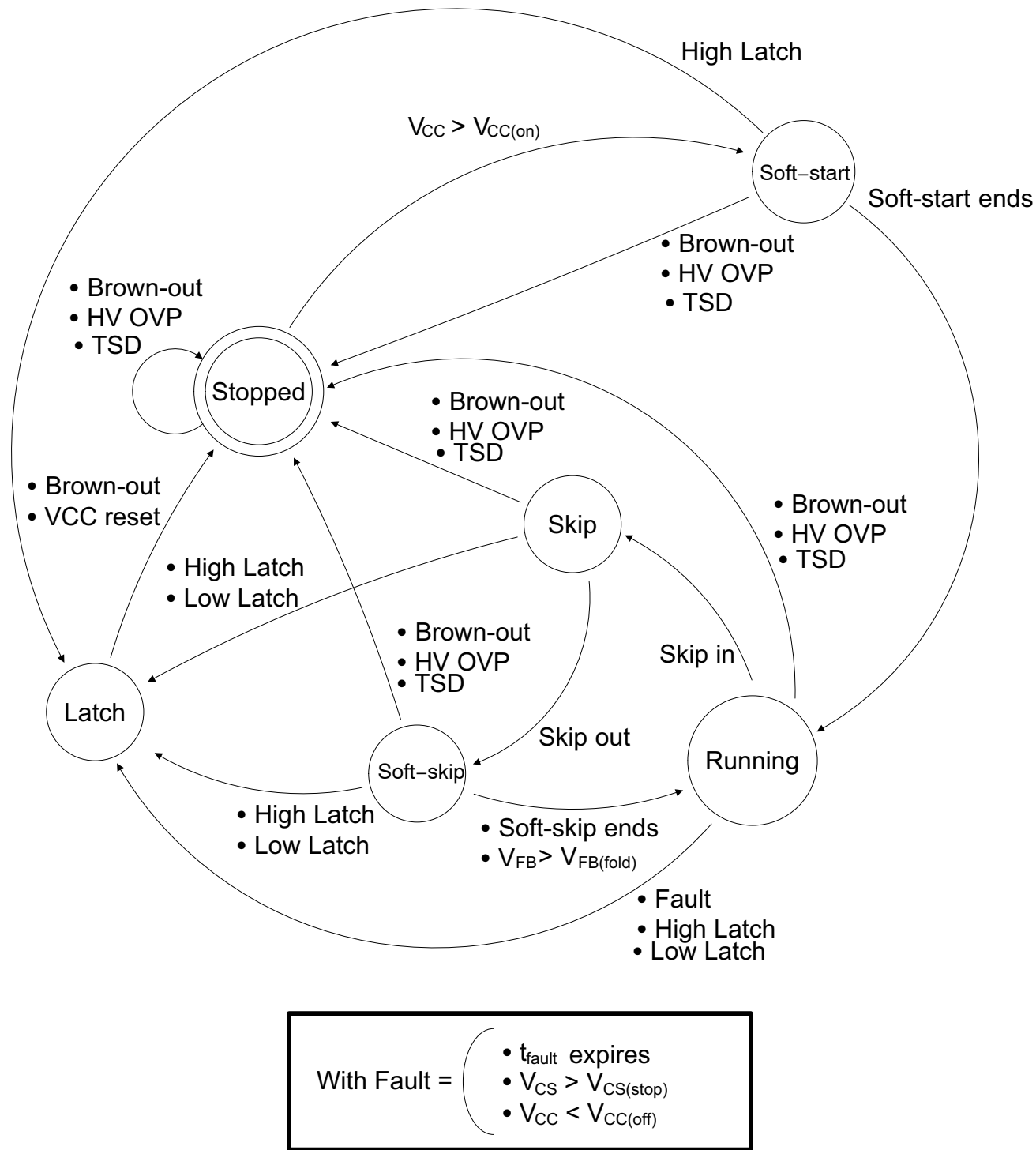
Figure 26. Controller Operation State Diagram (Latched Protection)
