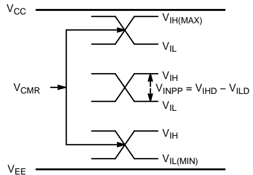
Figure 19. V_{CMR} Diagram
