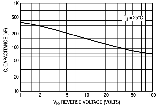
Figure 17. Typical Capacitance (Per Leg)
