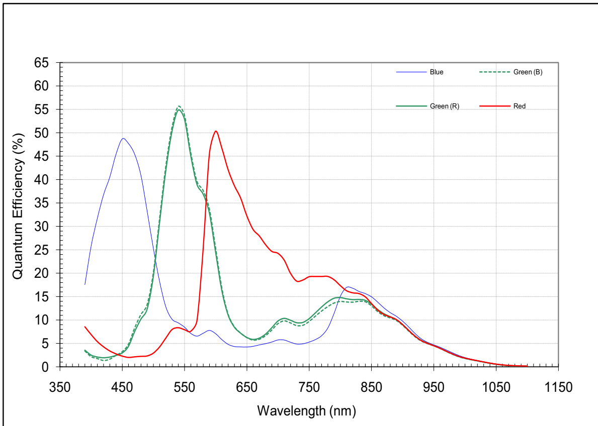
Figure 35: Typical Quantum Efficiency
