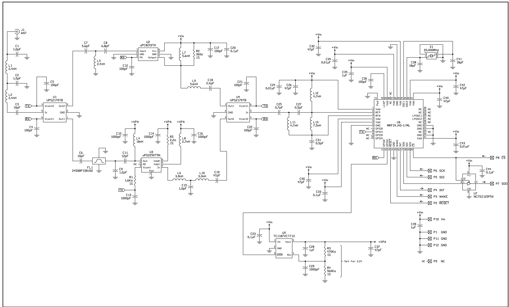
FIGURE 2-2: MRF24J40MC SCHEMATIC
