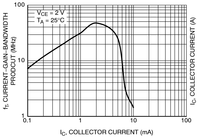
Figure 4. Current-Gain-Bandwidth Product
