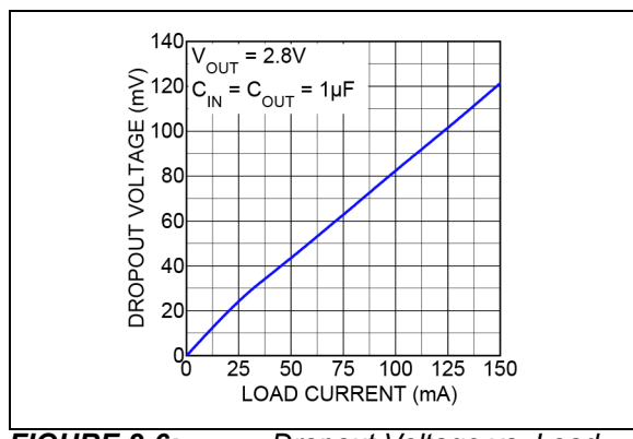
FIGURE 2-6: Dropout Voltage vs. Load Current.
