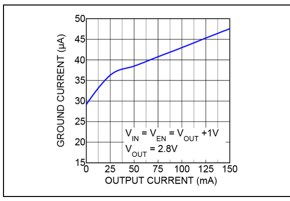
FIGURE 2-3: Ground Current vs. Output Current.
