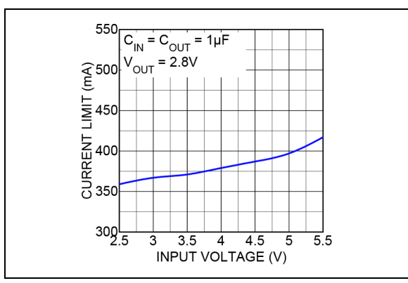
FIGURE 2-2: Current Limit vs. Input Voltage.
