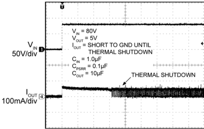
Time (100ms/div)
