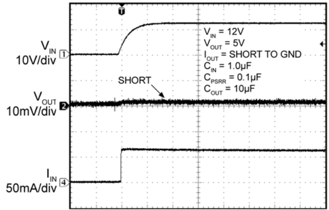
Time (40ms/div)
