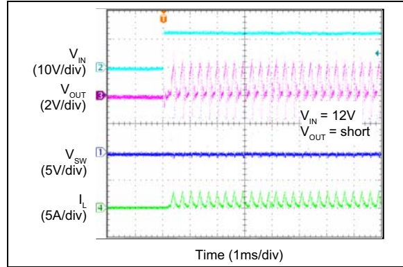
FIGURE 2-35: Turn-On Into Short-Circuit.
