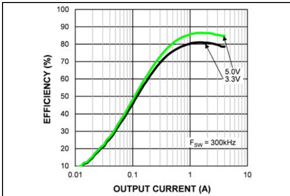
FIGURE 2-25: Efficiency ( V_{IN} = 36\text{V} ) vs. Output Current (MIC28513-2).
