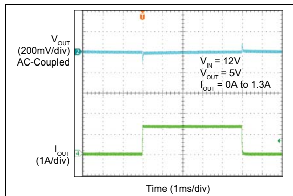
FIGURE 2-48: MIC28513-2 Transient Response (0A to 1.3A).
