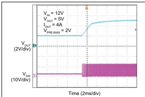
FIGURE 2-33: MIC28513-2 V_{IN} Start-Up with Pre-Biased Output.
