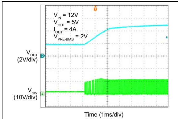
FIGURE 2-32: MIC28513-1 V_{IN} Start-Up with Pre-Biased Output.
