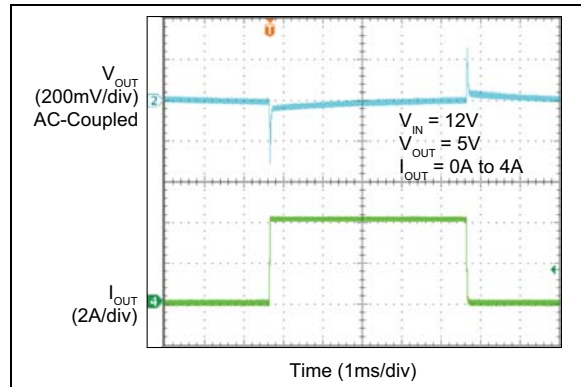
FIGURE 2-46: MIC28513-2 Transient Response (0A to 4A).
