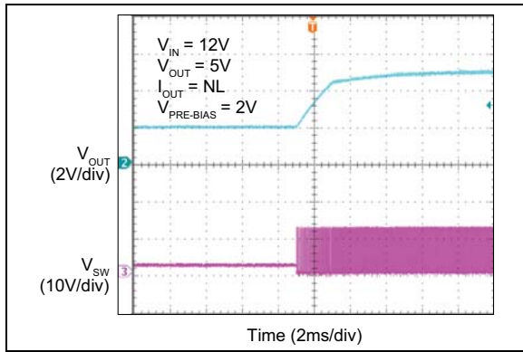
FIGURE 2-31: MIC28513-2 V_{IN} Start-Up with Pre-Biased Output.
