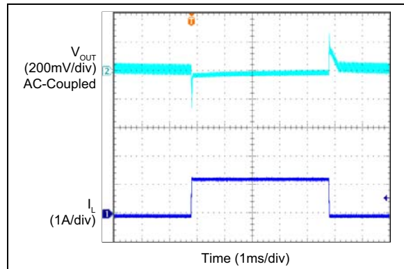
FIGURE 2-47: MIC28513-1 Transient Response (0A to 1.3A).
