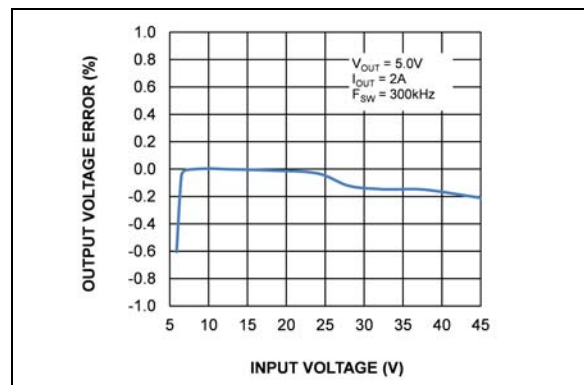
FIGURE 2-6: Line Regulation Error ( V_{OUT} vs. V_{IN} ).
