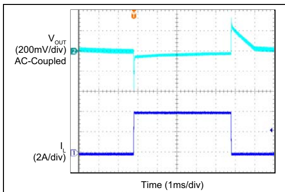
FIGURE 2-45: MIC28513-1 Transient Response (0A to 4A).
